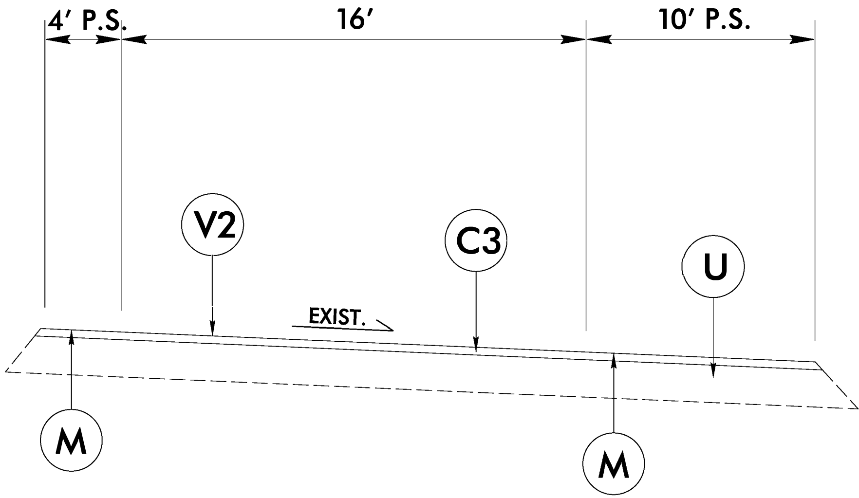
TYPICAL SECTION NO. 2
